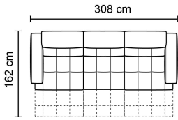
370 SECT.450+338+452
